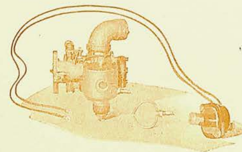
Complete Equipment Switch, Wires and Heater, also Heater in Carburetor.
