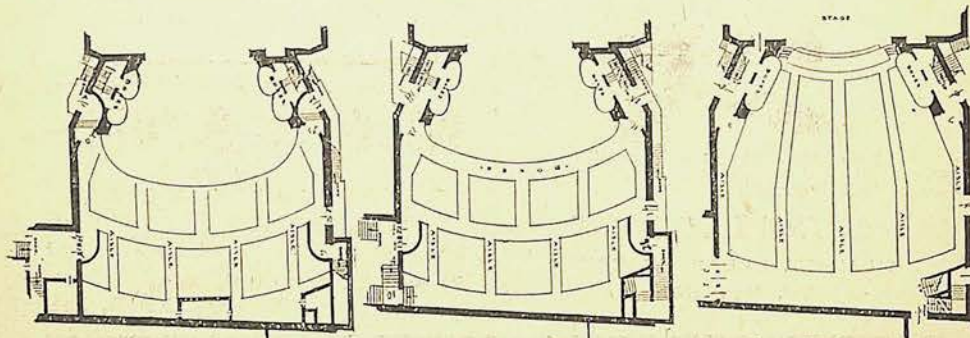
GROUND FLOOR
